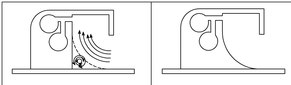
Figure 16: Flow vortices deflecting flow in the original design and "curved" inlet design.
