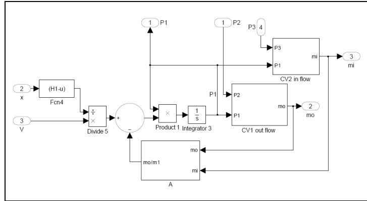
Figure C10: Subsystem A.
